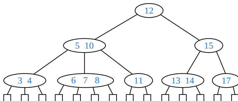
Figure 11.23: A (2,4) tree.
