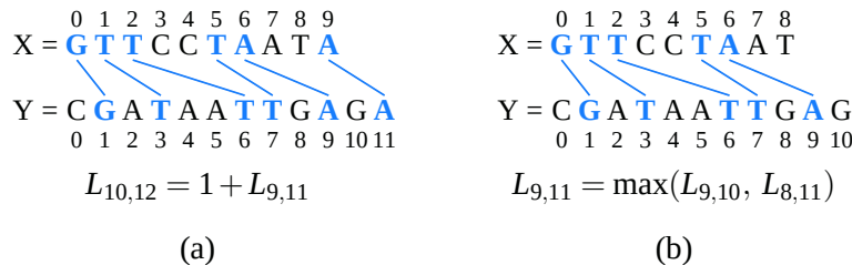
Figure 13.13: The two cases in the longest common subsequence algorithm for computing L_{j,k} when j, k \geq 1 : (a) x_{j-1} = y_{k-1} ; (b) x_{j-1} \neq y_{k-1} .
